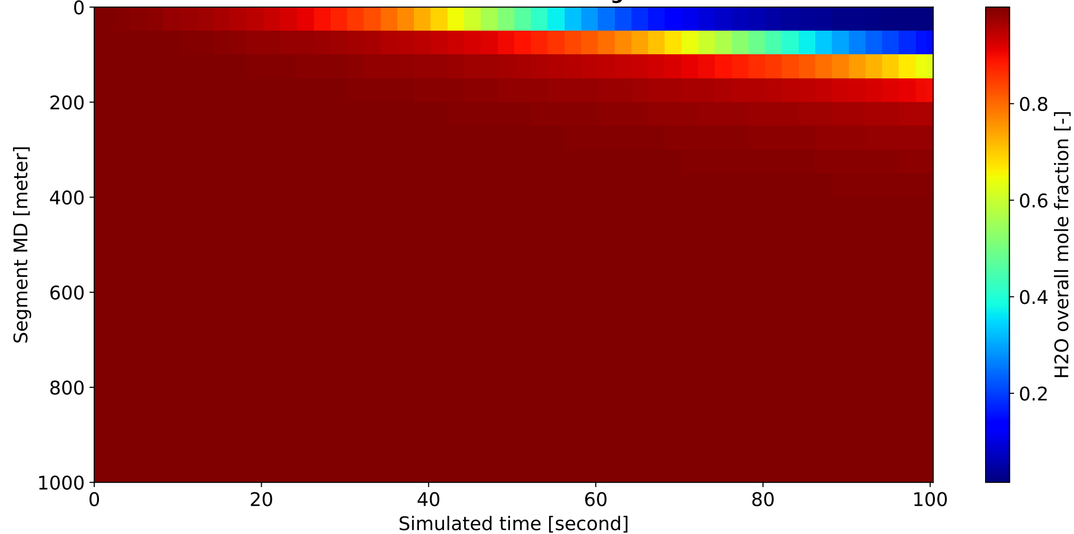
Profile of overall mole fraction of H 2 O along the wellbore over time
